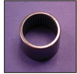
BEARING # 931 CHRYSLER LARGE 2/GEAR (32MM X 38MM X 18.8MM)
