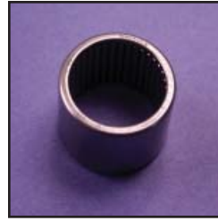
BEARING # 930 SAGINAW MODEL 605 2/GEAR (29MM X 35MM X 25MM)
