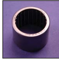
BEARING # 934 FORD SECTOR (34MM X 41.2MM X 31.6MM)
